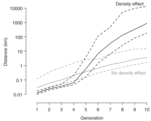
Fig. 7. Comparison of population spread resulting from density-dependent dispersal as predicted by the overall best inverse model (black), and from density-independent dispersal as predicted by the best standard model (grey). For 99 replicate simulations, the graphs indicate the medians (solid lines) and 95% confidence intervals (hatched lines) of the distance between the origin of spread and the furthest forward individual. Note that distances are plotted on a log-scale.
