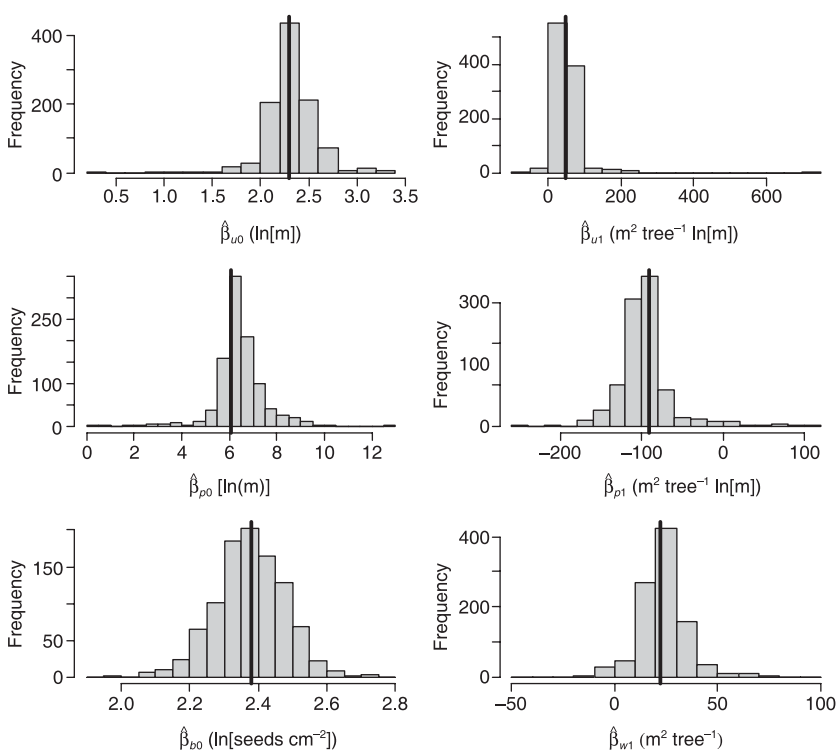
Fig. 5. Distribution of 999 bootstrapped parameter estimates for the selected inverse model that includes fecundity parameter \beta_{b0} , source effects on the shape and scale of a WALD dispersal kernel (described by intercepts \beta_{u0} and \beta_{p0} , and slopes \beta_{u1} and \beta_{p1} ), and a path effect (parameter \beta_{w1} ). The bold lines indicate maximum-likelihood parameter estimates.
