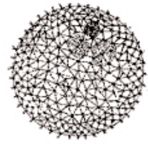
Volvox
